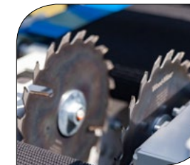
Two circular 25 cm blades - one fixed, and the other adjustable
